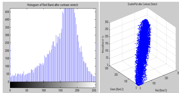
Fig. 5 Histogram and Scatterplot after Contrast Stretch
